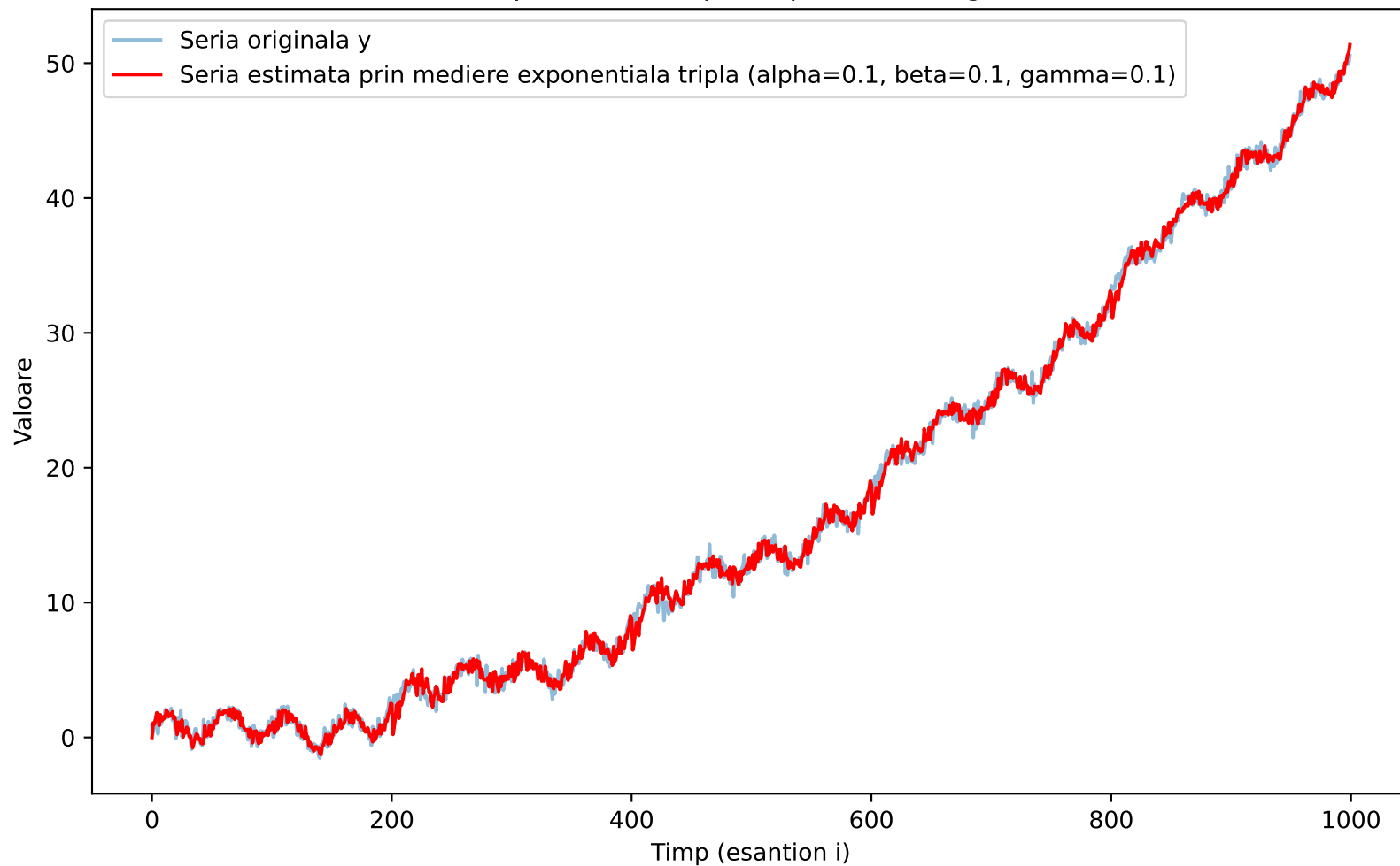
Medierea exponentiala tripla, alpha, beta si gamma fixate
